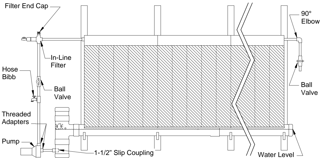
Figure 19 — 40' to 60' Centrifugal Pump System
