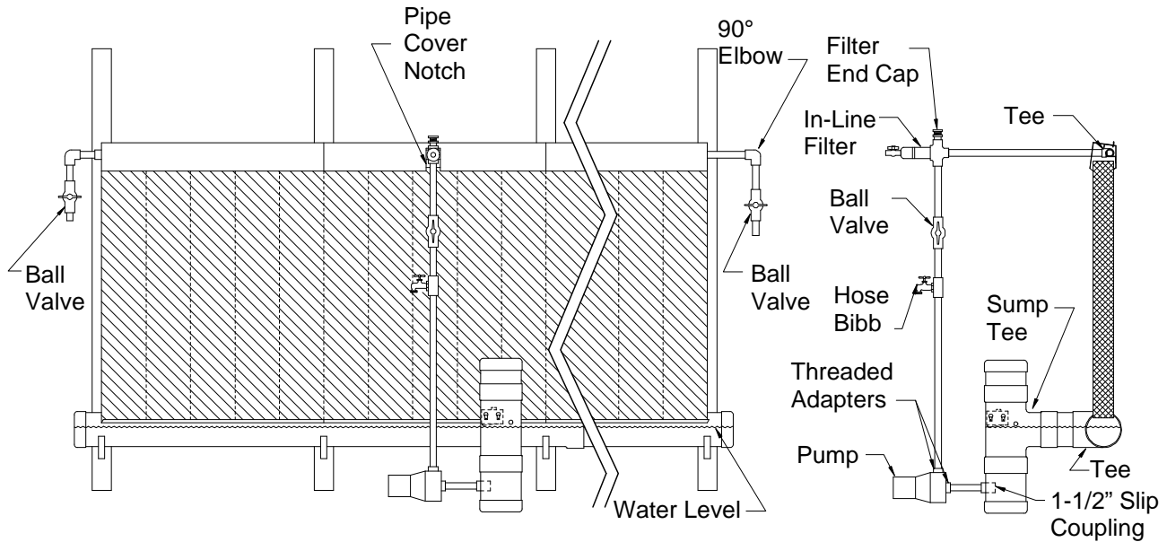
Figure 20 — 65' to 110' Centrifugal Pump System
