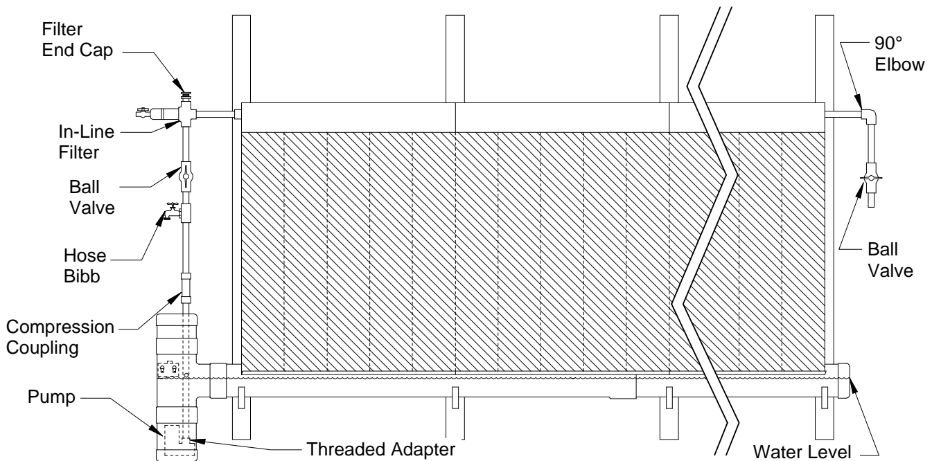
Figure 17 — 5' to 60' Submersible Pump System
