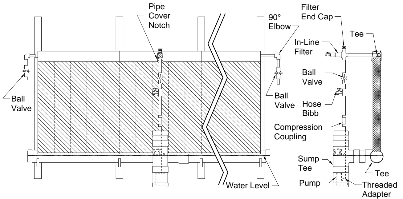
Figure 18 — 65' to 70' Submersible Pump System
