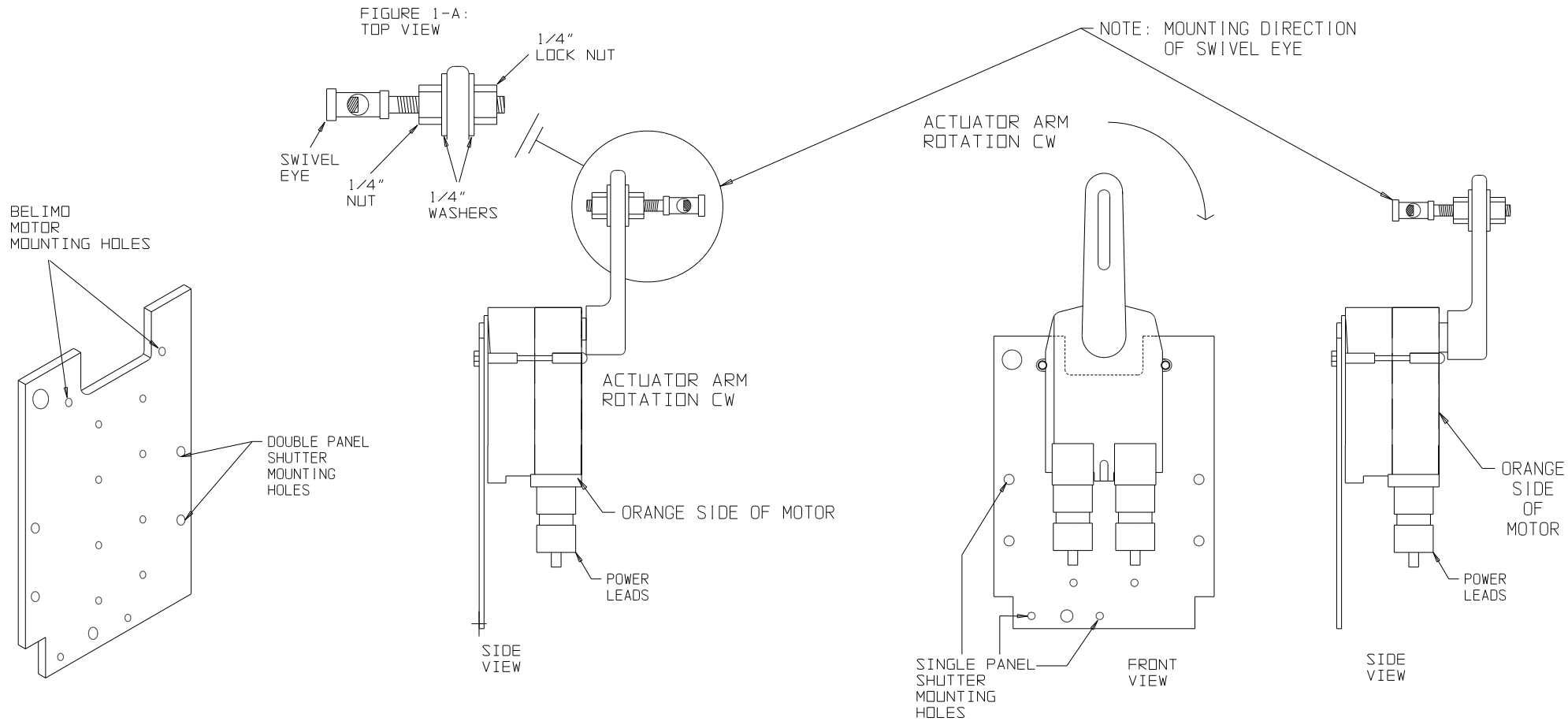
FIGURE 1: DOUBLE PANEL S-SHUTTER & LRW 39-66
