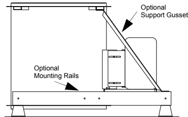
Figure 5 Vertical Floor Mount (shown discharge down)
