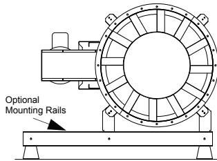
Figure 3 Horizontal Base Mount Motor at 3 or 9 o'clock position
