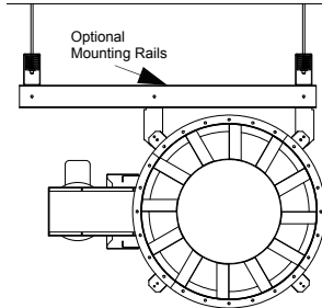
Figure 3 Horizontal Base Mount Motor at 3 or 9 o'clock position
