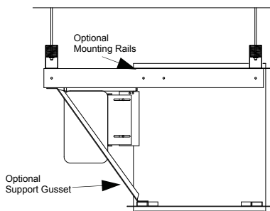
Figure 6 Vertical Ceiling Mount (shown discharge up)
