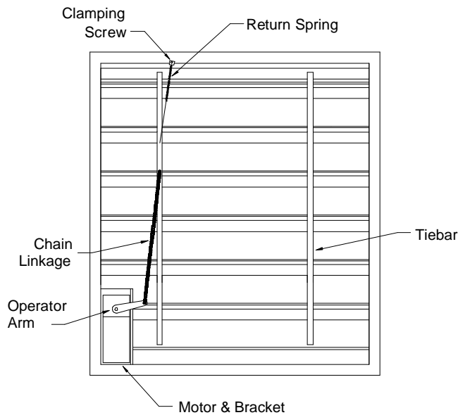
FS24 - FS36 Motorized Shutter
