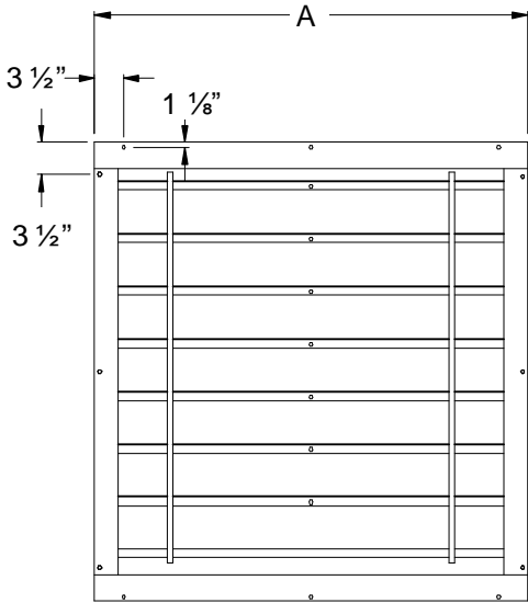
Rear View Automatic Shutter (Closed)
