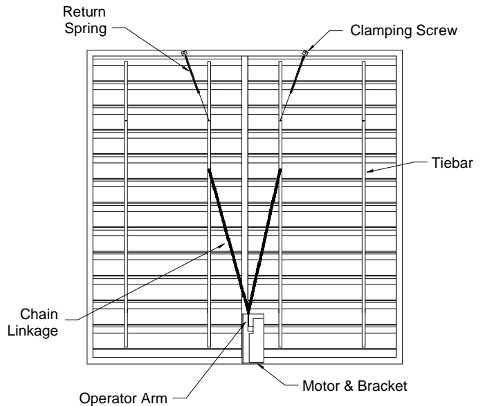
FS42 - FS54 Motorized Shutter
